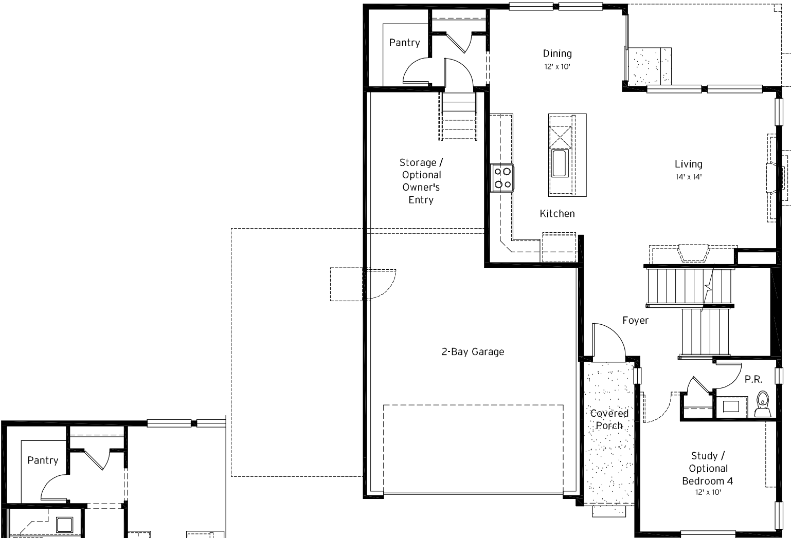
Main Level Floor Plan
