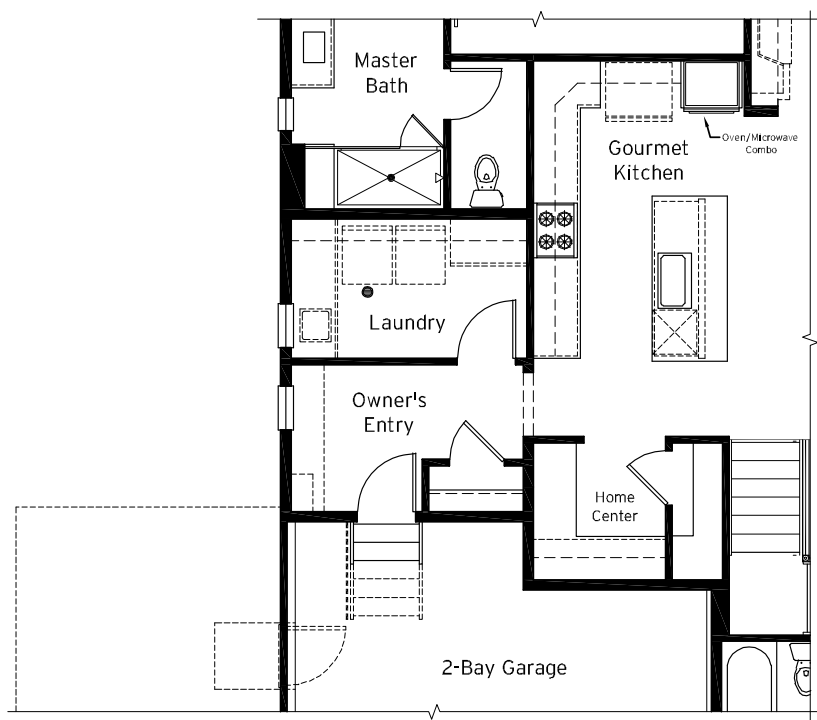
Optional Owner's Entry
