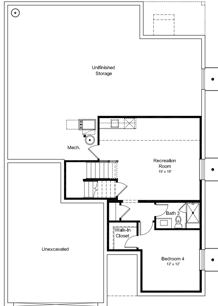
Opt. Finished Lower Level w/ Storage Floor Plan
