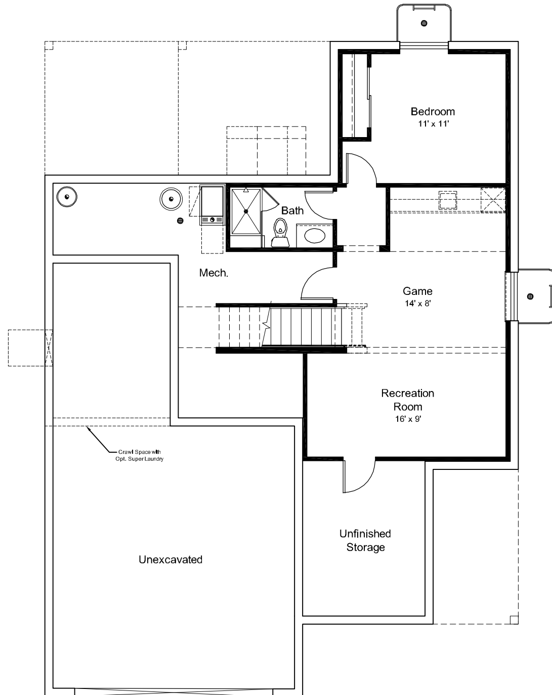
Lower Level Floor Plan
