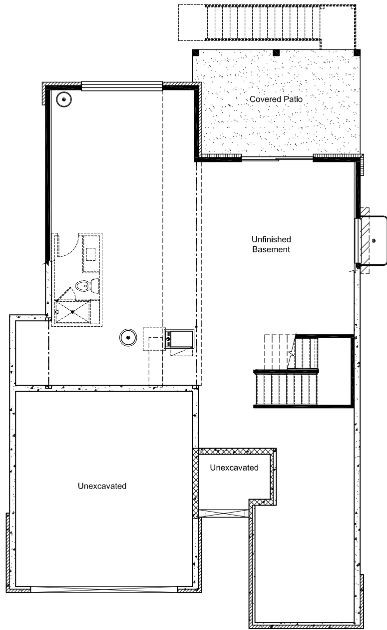
Unfinished Lower Level Floor Plan
