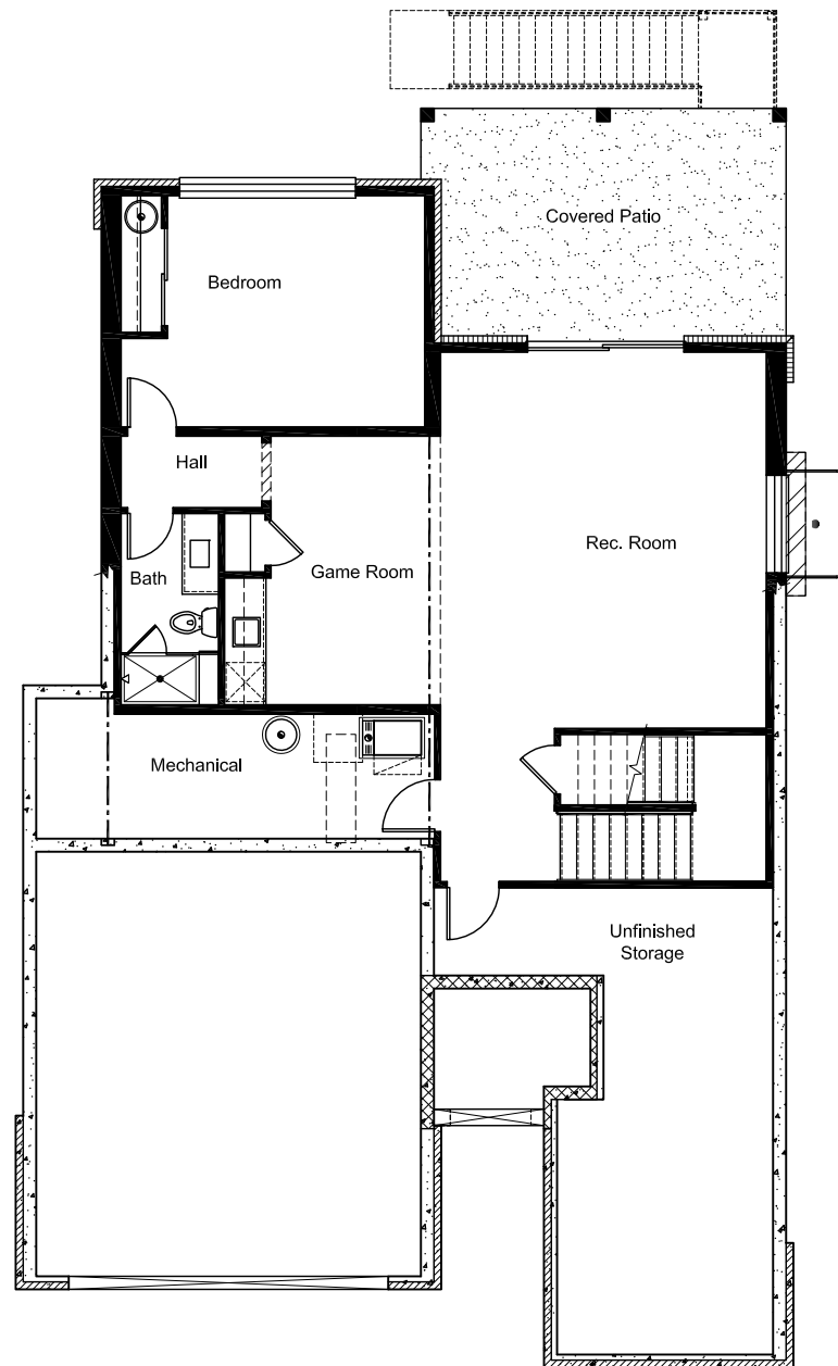
Opt. Finished Lower Level Floor Plan
